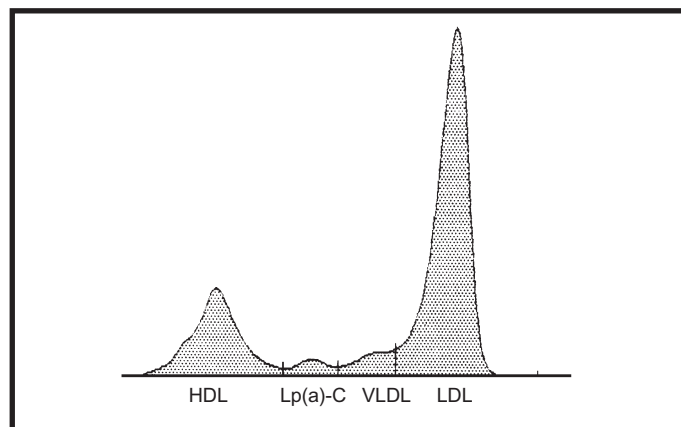
Figure 1: A scan of a SPIFE Cholesterol pattern.
